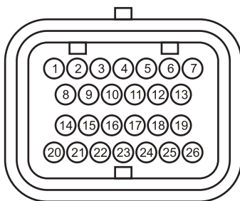
ECU CONNECTOR (26 PIN) (Looking into ECU)
