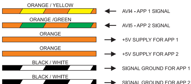
Figure 6 - Accelerator Pedal Position Sensor Wiring
