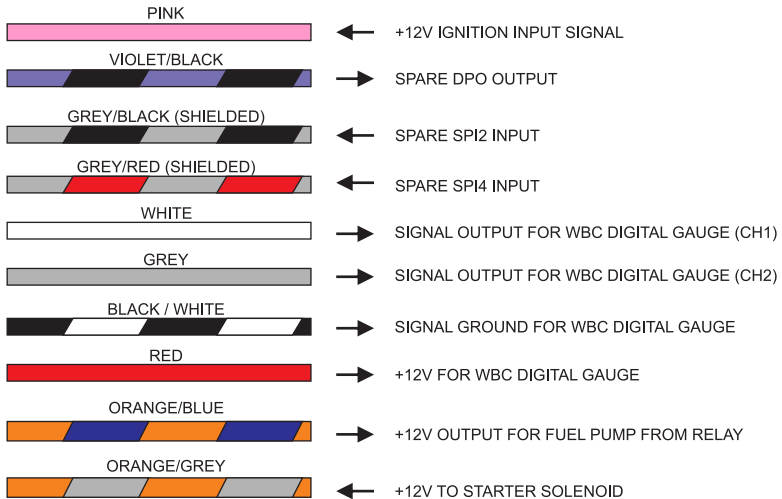
Figure 5 - Cabin Harness Wiring
