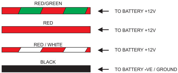
Figure 7 - Battery Wiring
